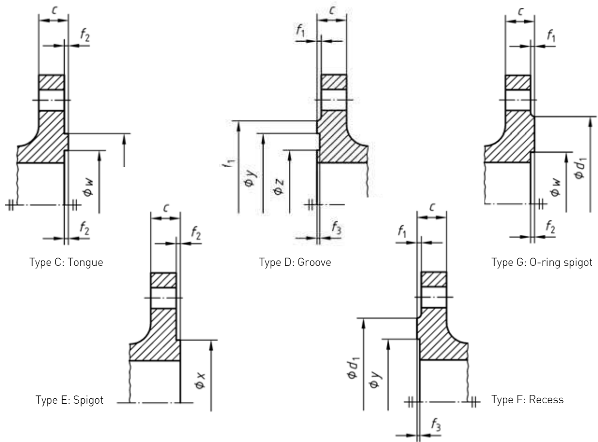
Flange connections according to EN 1092-1
