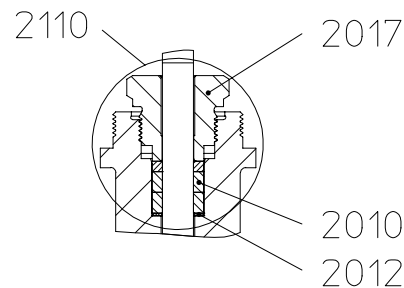
III. Stainless steel-bellows with pure graphite-packing
