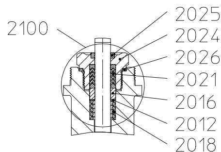
III. Stainless steel-bellows with V-ring unit
